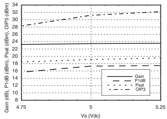
Gain, Power & OIP3 vs. Supply Voltage for R_s = 18 \text{ Ohms} @ 850 MHz
