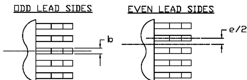
DETAIL "A"
