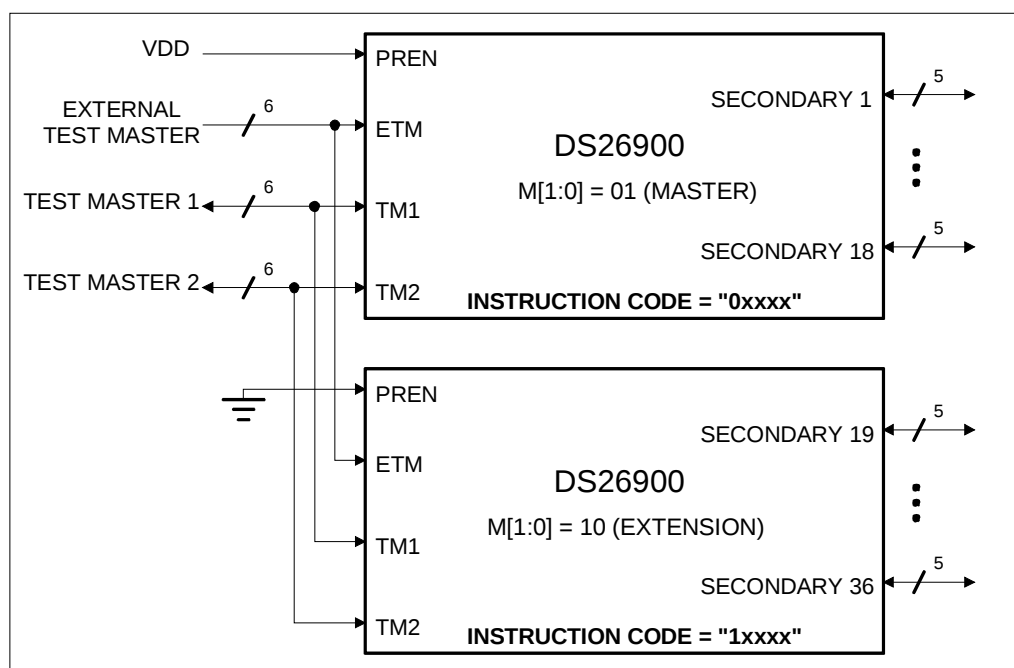
Figure 4-3. Two Cascaded Devices
