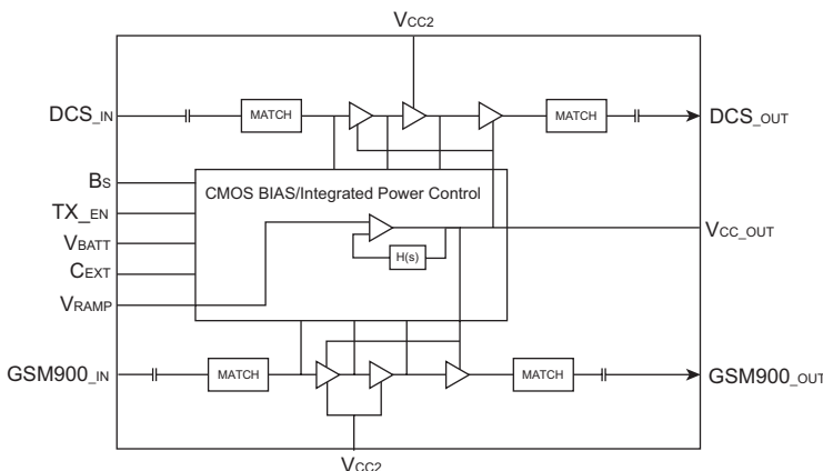
Figure 1: Block Diagram
