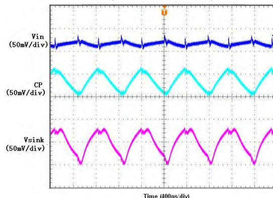
Load Characteristics ( V_{IN} = 2.7V ; 2X Mode; 14mA Load)
