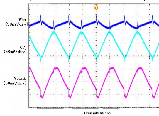
Load Characteristics ( V_{IN} = 3.1V ; 2X Mode; 30mA Load)
