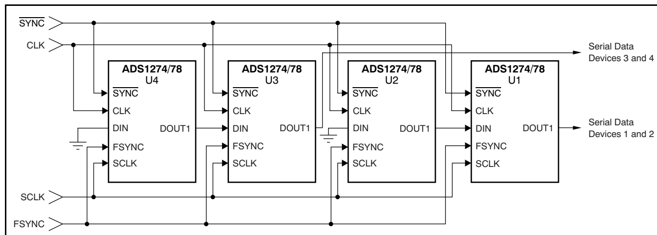
Figure 82. Daisy-Chain Data Format of Figure 81 (ADS1278 shown)
