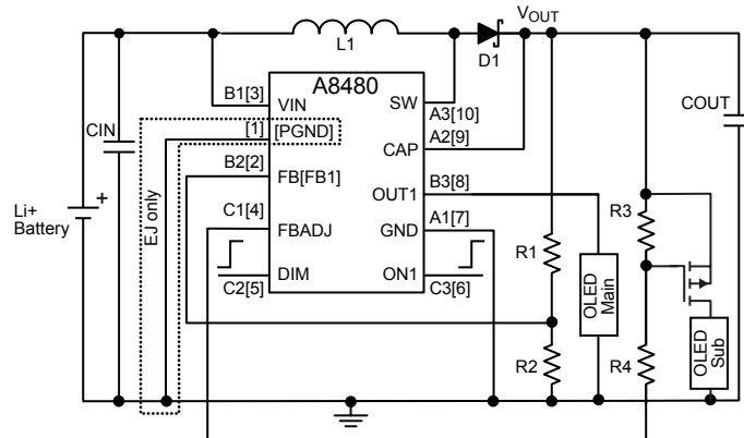
Figure 5. Main and sub OLED bias with both grounded
