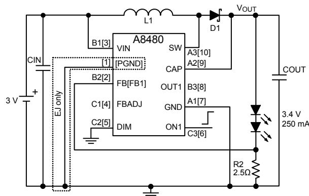
Figure 7. A8480 driving high current flash/torch LEDs
