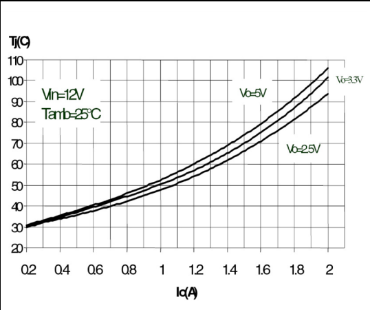
Figure 9. Junction temperature vs. output current
