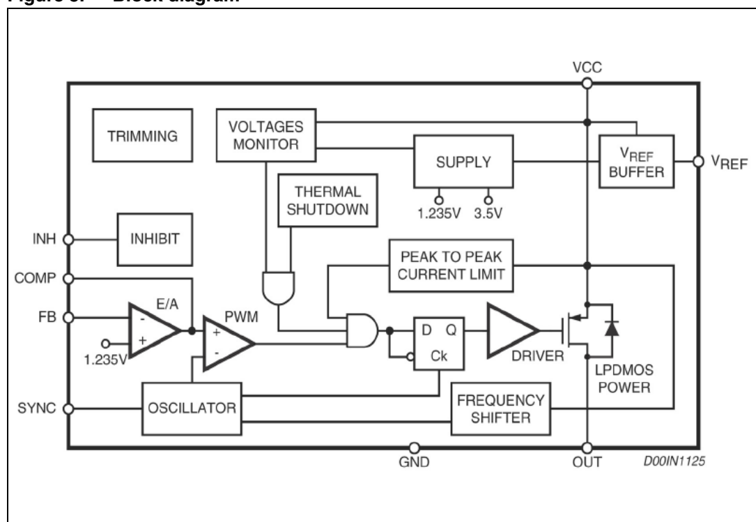
Figure 3. Block diagram
