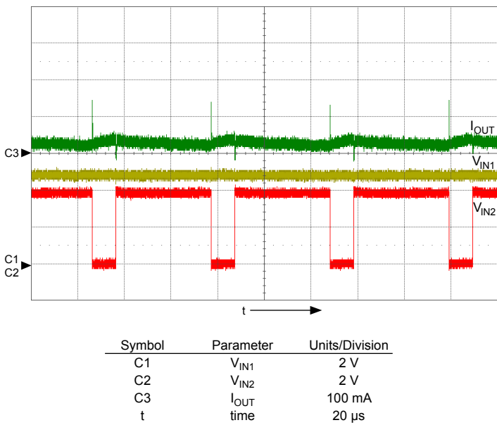
Figure 2. Enable chopping. Forward direction, duty cycle 10%.
