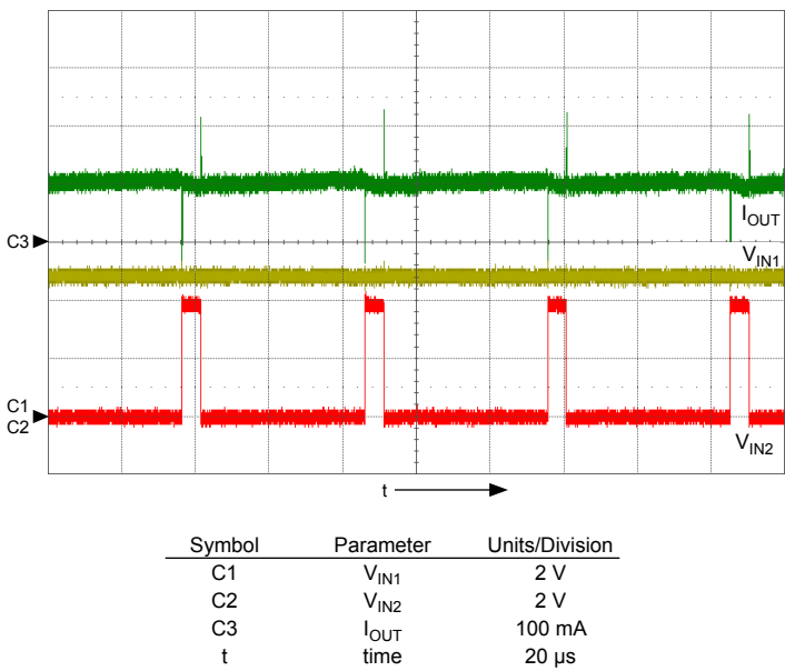
Figure 1. Enable chopping. Forward direction, duty cycle 90%.
