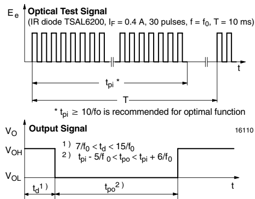
Figure 1. Output Function
