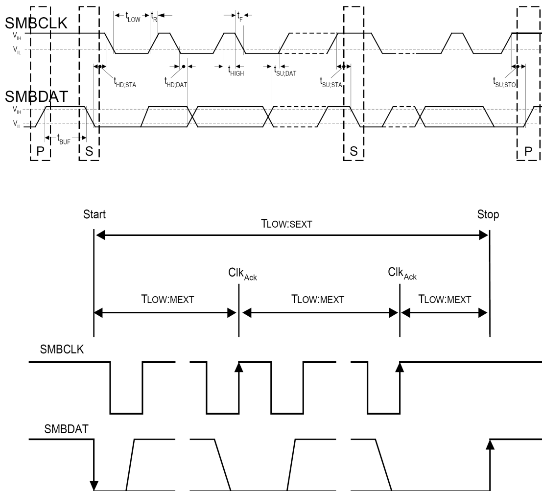
Figure 1 I 2 C/SMBus/PMBus Timing Diagram
