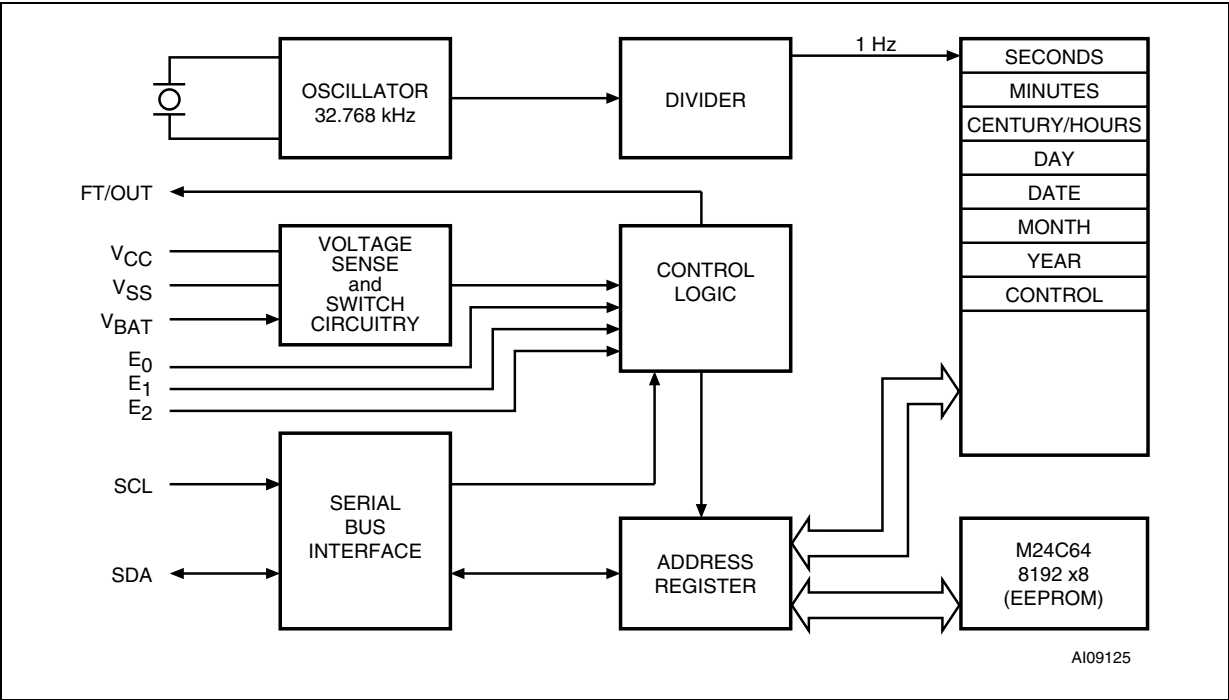
Figure 3. Block diagram
