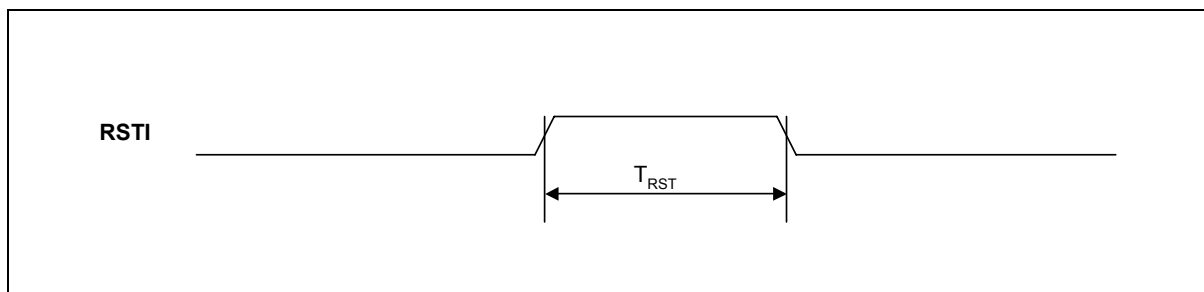
Figure 5.1 RESET Timing Diagram
