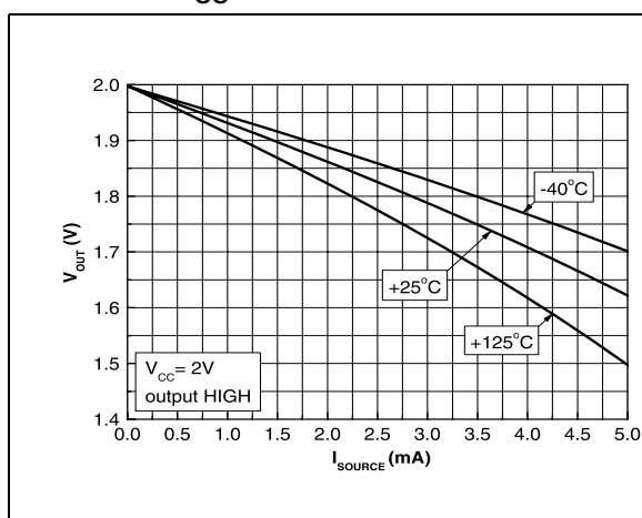
Figure 5. Output voltage vs. source current V_{CC}=2V
