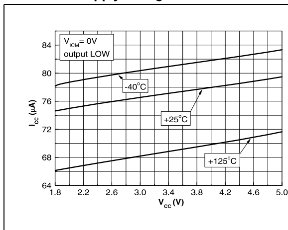
Figure 3. Current consumption vs. power supply voltage
