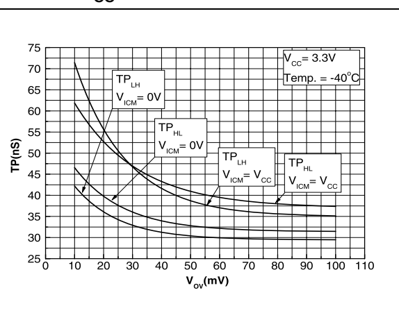
Figure 18. Propagation delay vs. overdrive V_{CC}=3.3V
