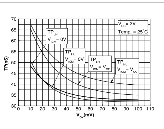
Figure 14. Propagation delay vs. overdrive V_{CC}=2V
