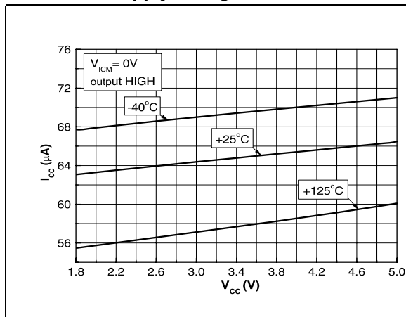
Figure 1. Current consumption vs. power supply voltage
