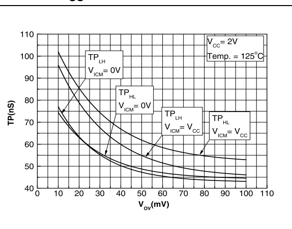
Figure 16. Propagation delay vs. overdrive V_{CC}=2V
