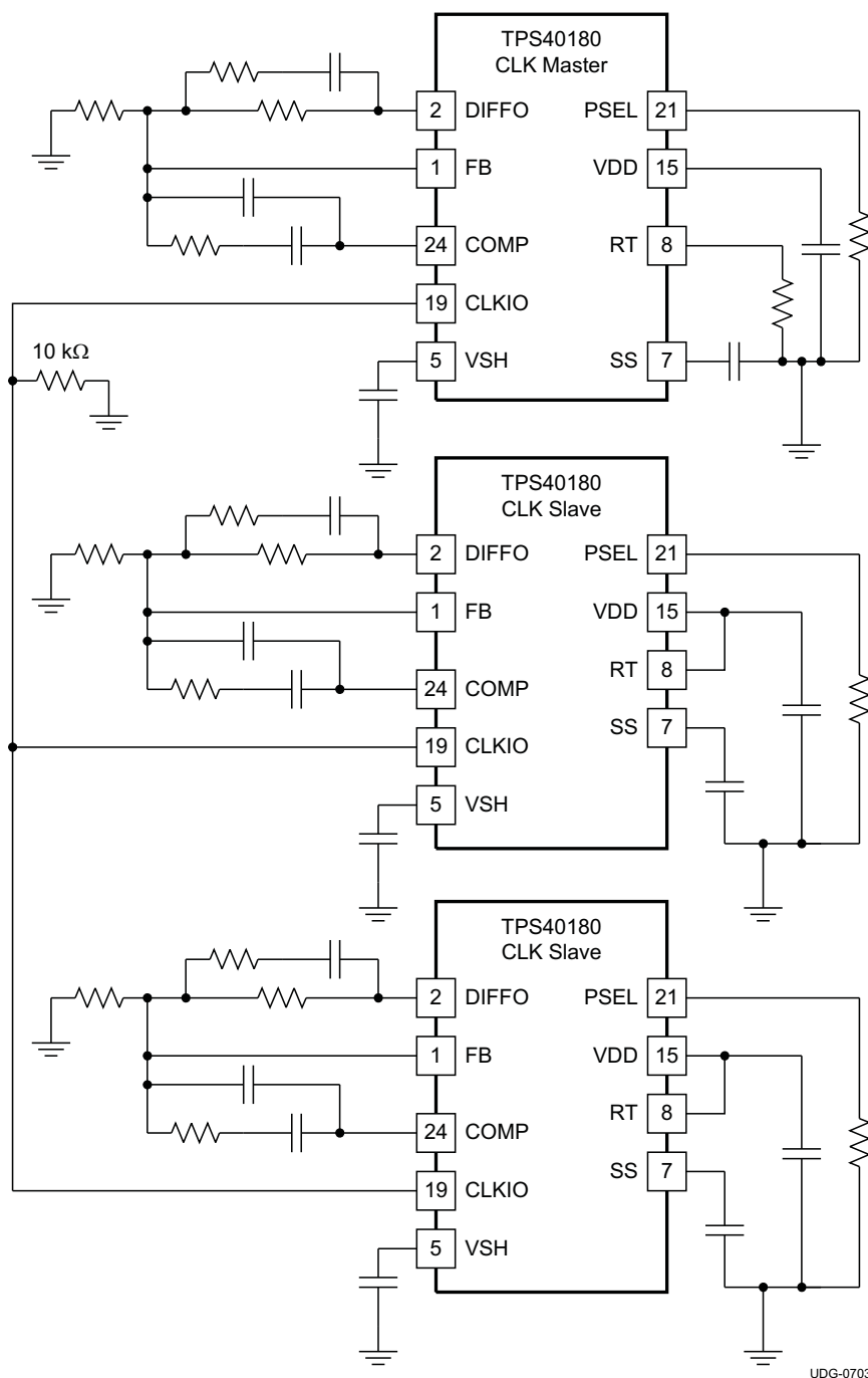
Figure 32. Phase Share Multiple Output Configuration
