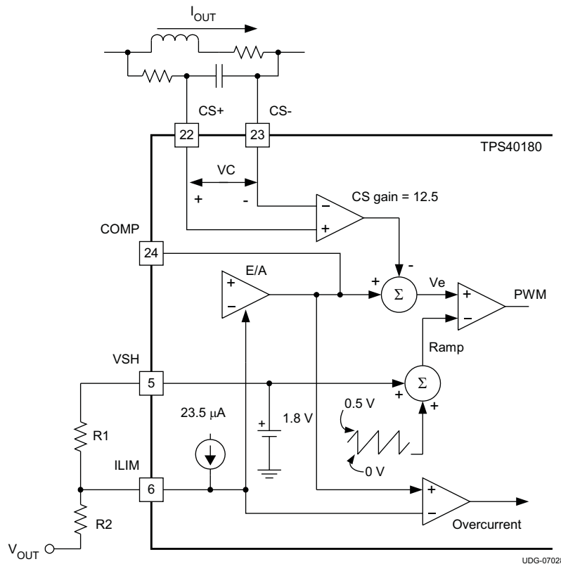
Figure 25. Current Sense Architecture
