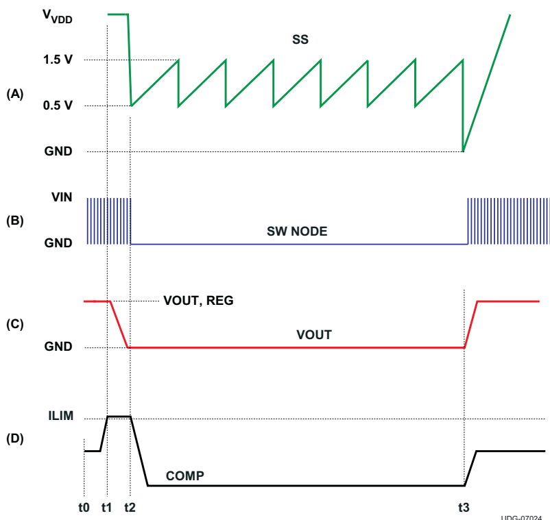
Figure 26. Hiccup Recovery From Faults
