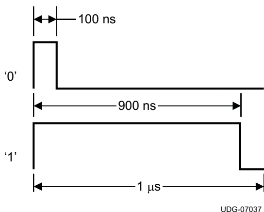
Figure 29. eTrim™ Bit Pulse Timing
