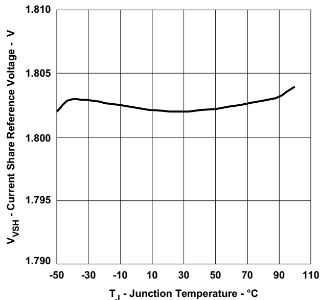
CURRENT SHARE RE VOLTAGE vs JUNCTION TEMPERATURE
