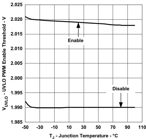
UVLO PWM ENABLE THRESHOLD VOLTAGE vs JUNCTION TEMPERATURE
