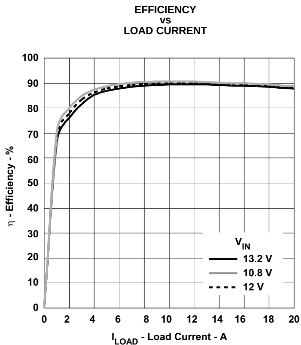
Figure 38. Efficiency Curve
