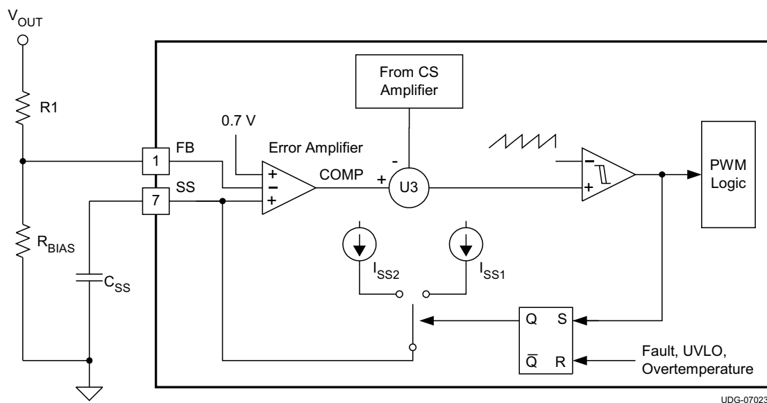
Figure 23. Soft-Start Implementation
