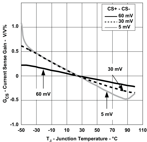
RELATIVE CURRENT SENSE GAIN vs JUNCTION TEMPERATURE
