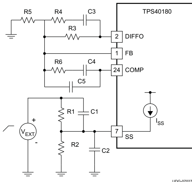
Figure 24. Tracking Setup
