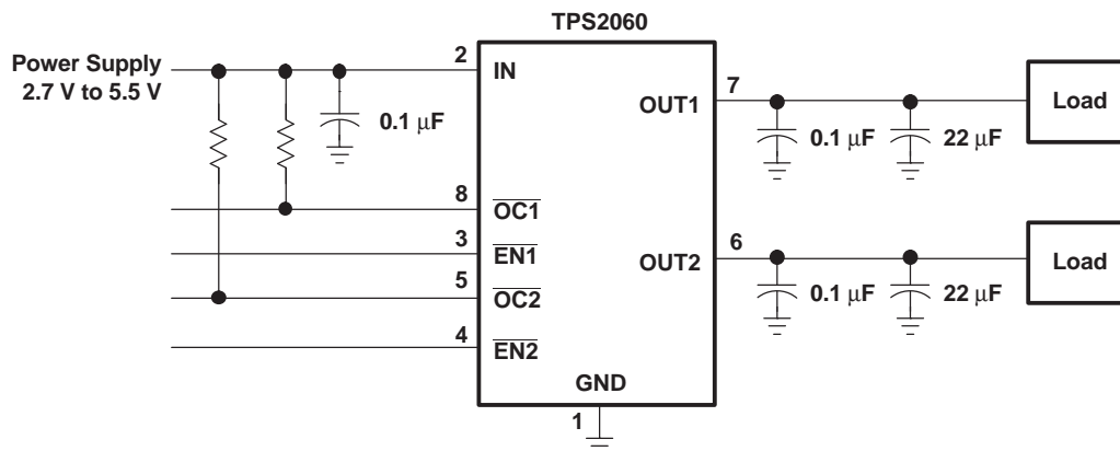
Figure 20. Typical Application
