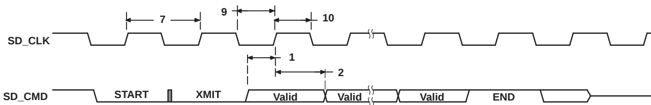
Figure 5-41. MMC/SD/SDIO Card Response Timing
