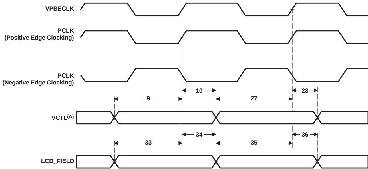
Figure 5-49. VPBE Input Timing With Respect to PCLK and VPBECLK
