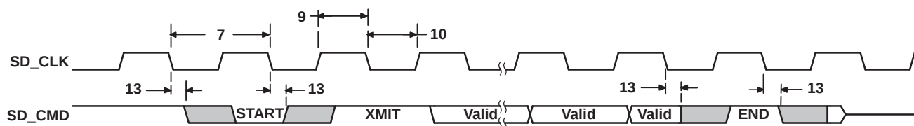
Figure 5-40. MMC/SD/SDIO Host Command Timing
