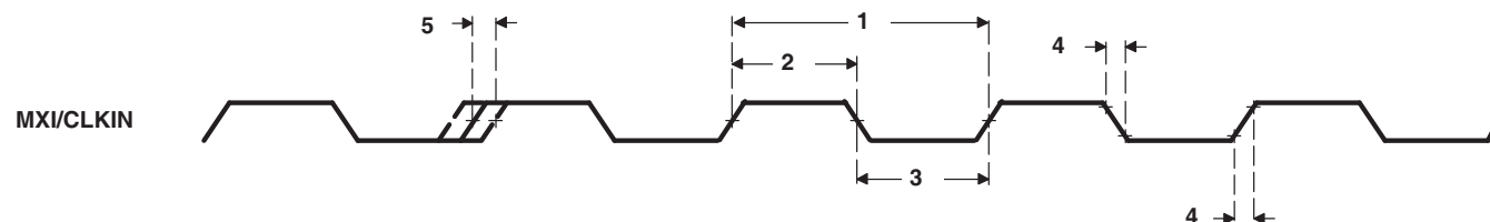
Figure 5-12. MXI/CLKIN Timing
