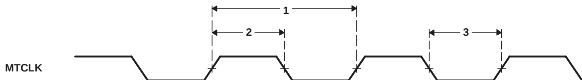
Figure 5-64. MTCLK Timing (EMAC - Transmit)
