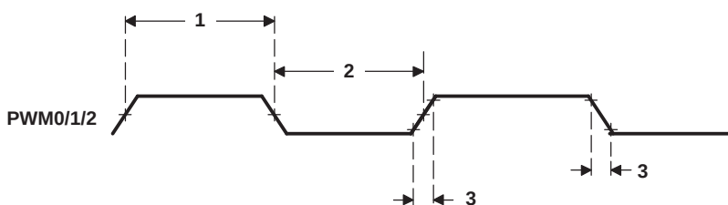
Figure 5-70. PWM Output Timing
