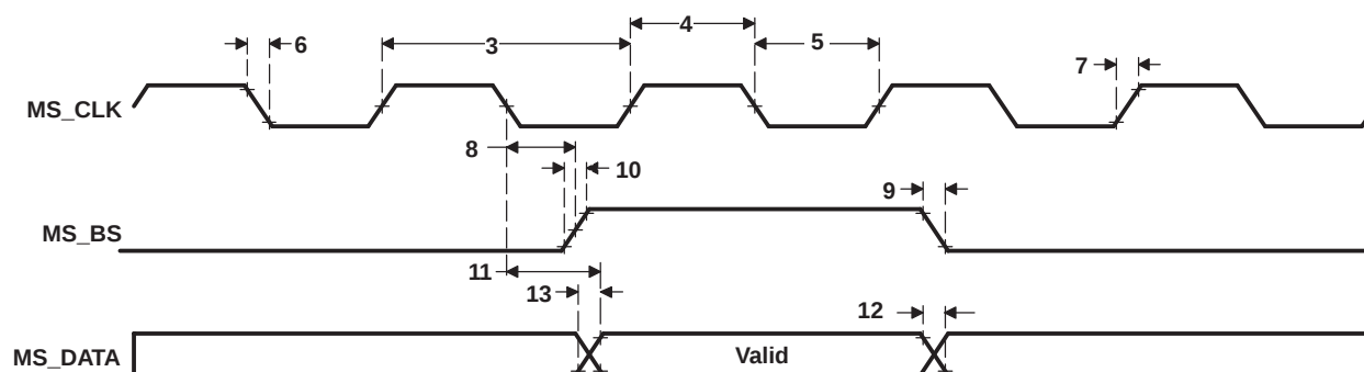
Figure 5-77. MS/MS PRO Parallel Interface Output Timing
