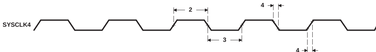
Figure 7-22. SYSCLK4 Timing
