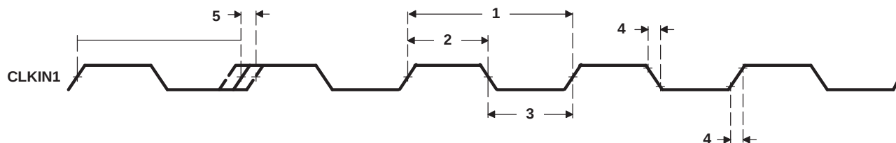
Figure 7-21. CLKIN1 Timing
