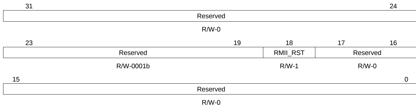
Figure 3-8. EMAC Configuration Register (EMACCFG) - 0x02AC 0020
