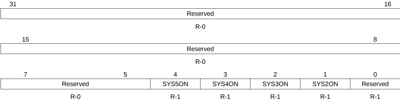
Figure 7-20. SYSCLK Status Register (SYSTAT) [Hex Address: 029A 0150]
