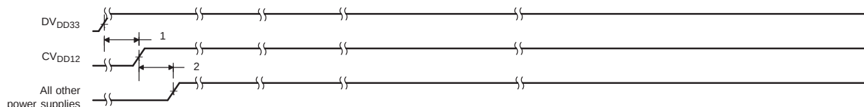
Figure 7-5. Power-Supply Sequence
