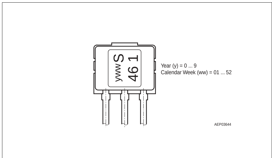
Figure 5 Marking TLE4946-1L
