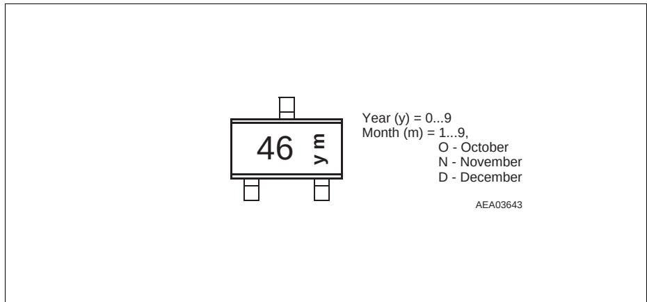
Figure 4 Marking TLE4946H
