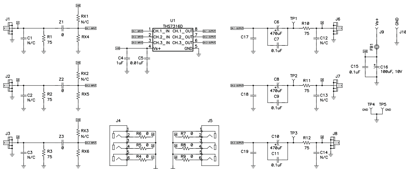
Figure 33. THS7316D EVM
