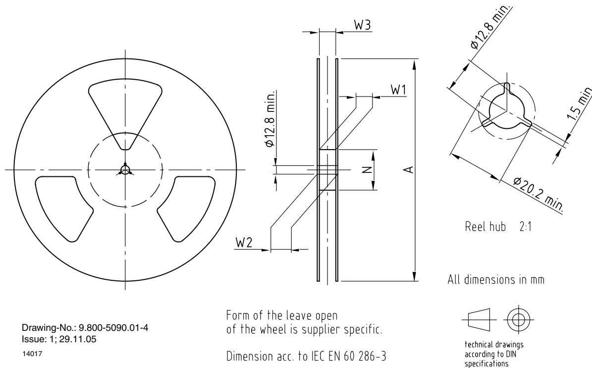
Figure 10. Reel dimensions, tolerance \pm 0.2 \text{ mm} , if not otherwise mentioned
