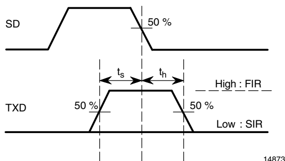
Figure 3. Mode Switching Timing Diagram
