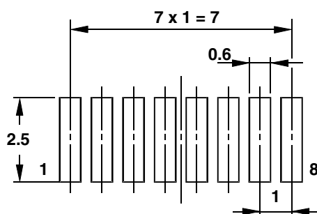
Figure 9. Recommended solder pad layout
