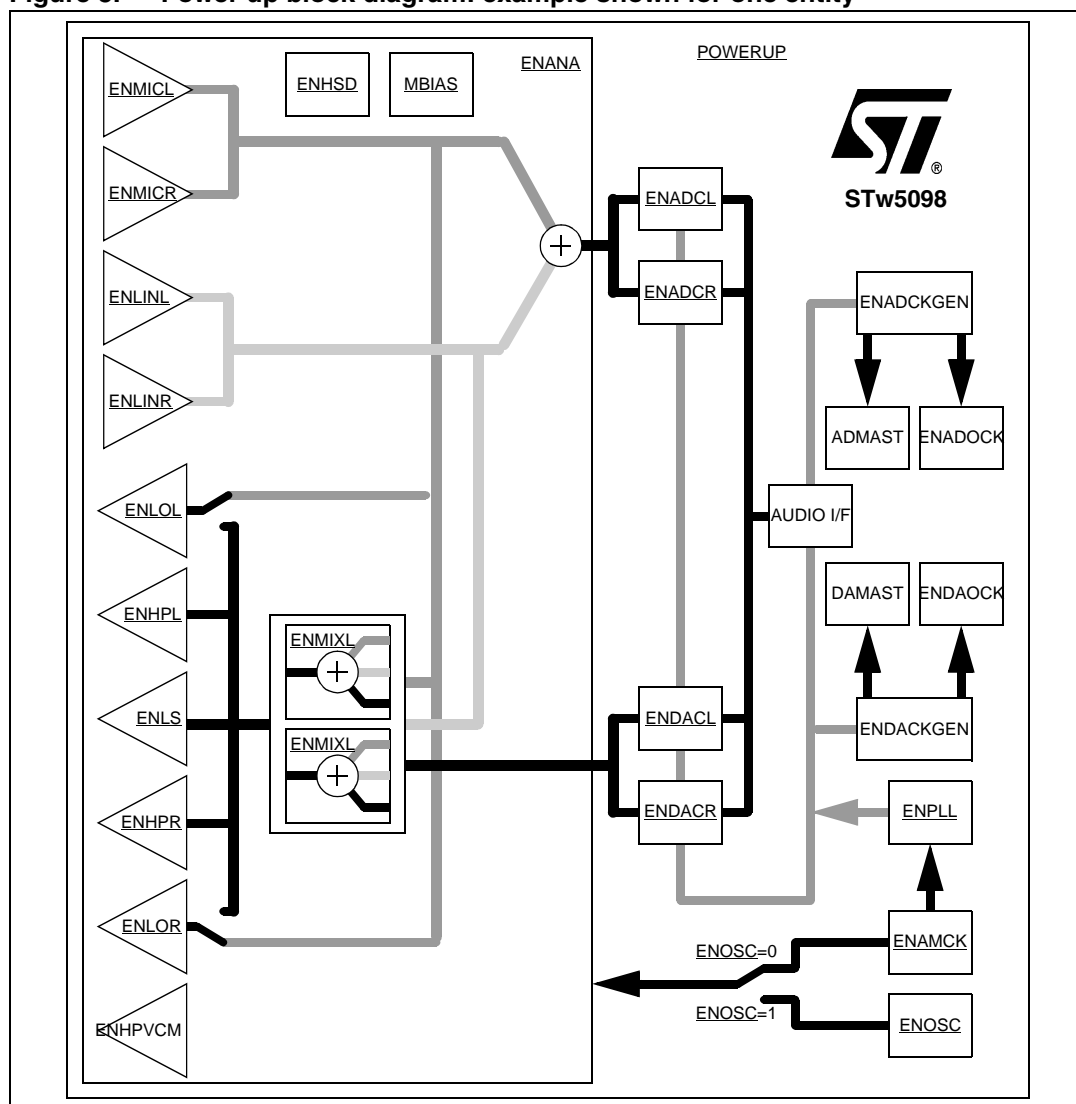
Figure 3. Power up block diagram: example shown for one entity
