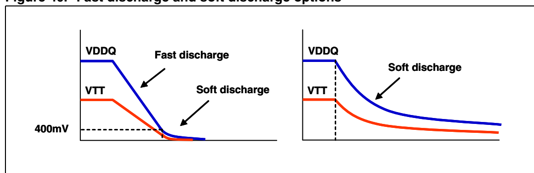
Figure 40. Fast discharge and soft discharge options
