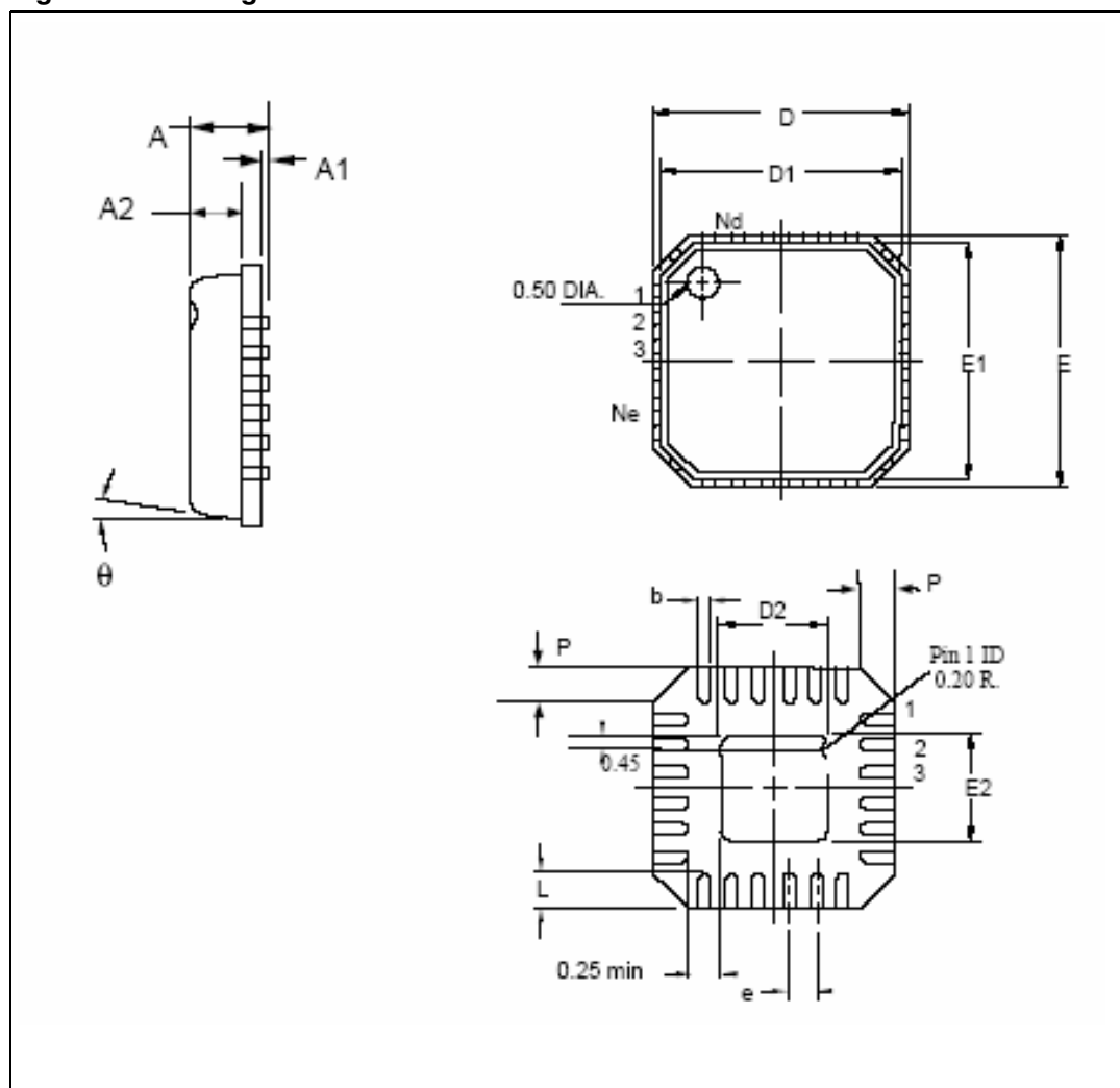
Figure 44. Package dimensions
