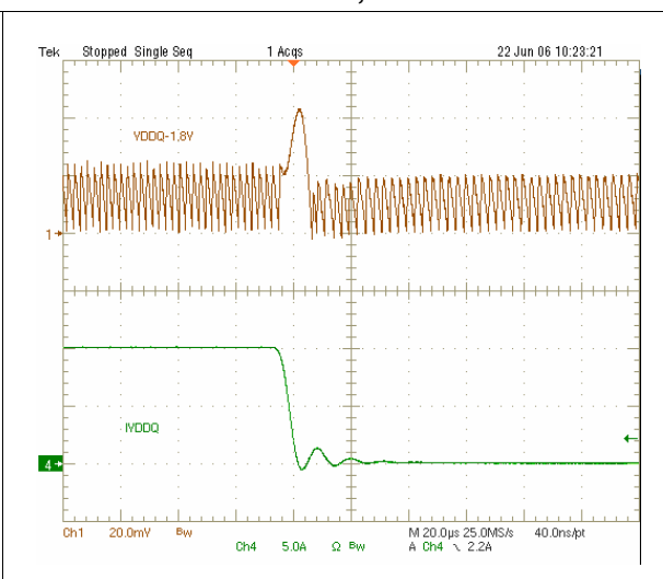
Figure 22. 10A to 0A VDDQ load transient, PWM
