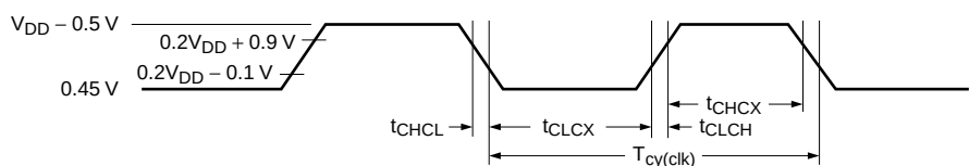
Fig 39. External clock drive waveform
