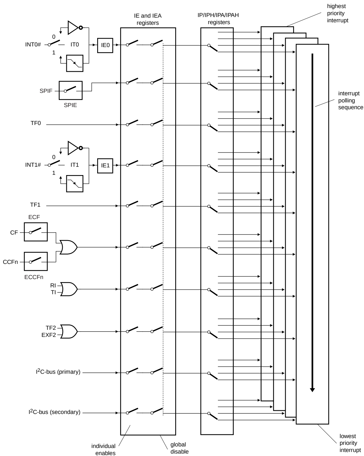
Fig 32. Interrupt structure
