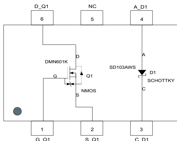
Fig 2 : Schematic and Pin Configuration
