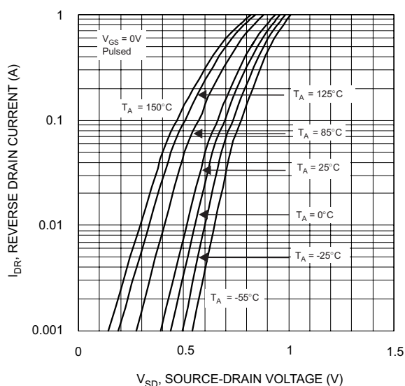
Fig. 11 Reverse Drain Current vs. Source-Drain Voltage
