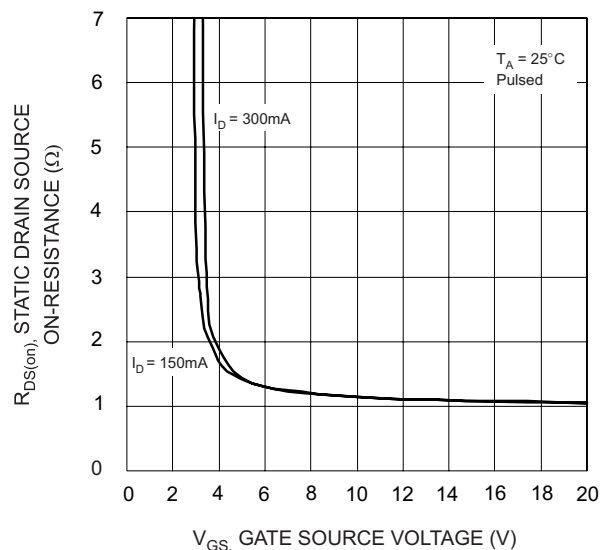
Fig. 9 Static Drain-Source On-Resistance vs. Gate-Source Voltage
