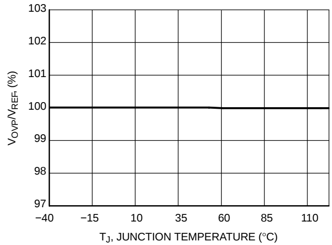
Figure 5. Ratio Overvoltage Threshold Overvoltage Reference vs. Temperature
