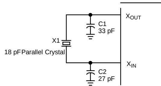
Figure 9. Crystal Input Interface
