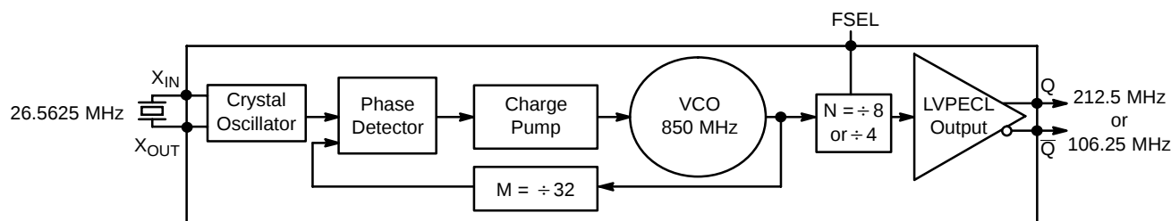
Figure 1. Logic Diagram
