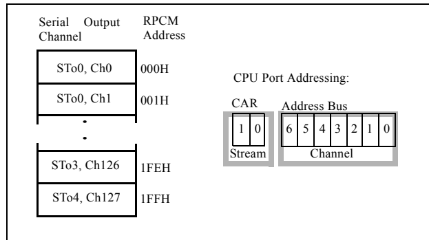
Figure 14b - 8.196 Mbps RPCM Addressing
