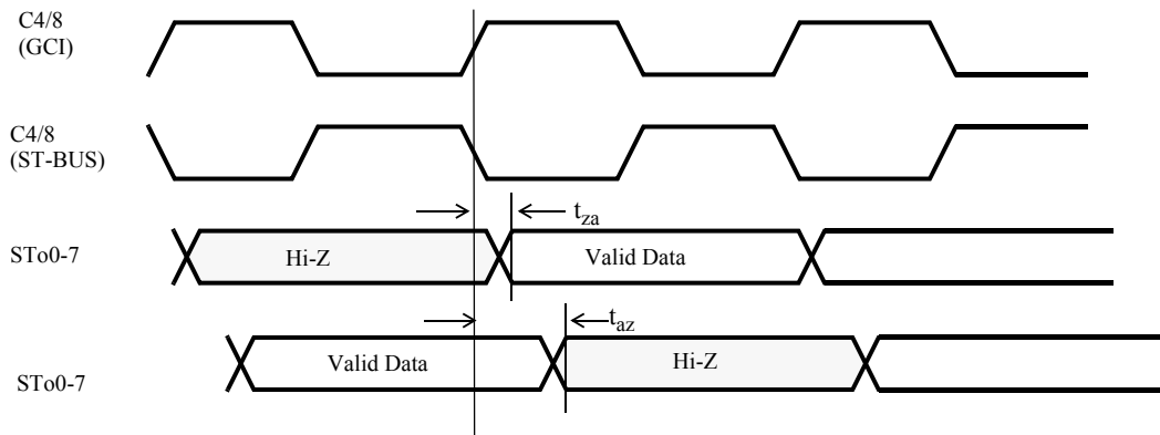
Figure 23 - Per-Channel Tristate Characteristics at all Data Rates
