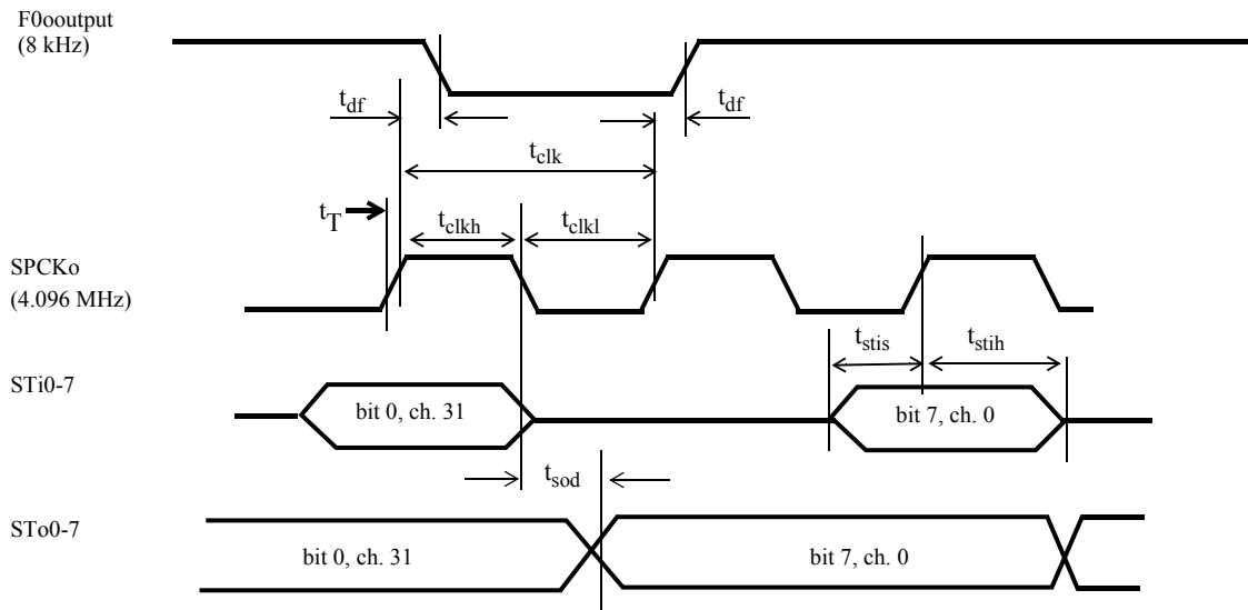
Serial Port with Negative Polarity F0 (ST-BUS)
