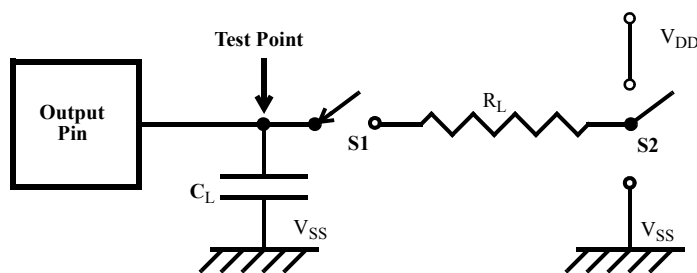
Figure 17 - Output Test Load
