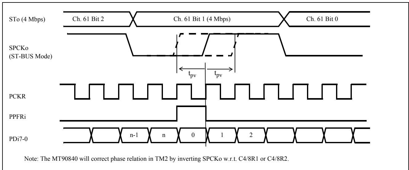
Figure 31 - Phase Variation Between C4 and PCKR Inputs for TM2 Operation
