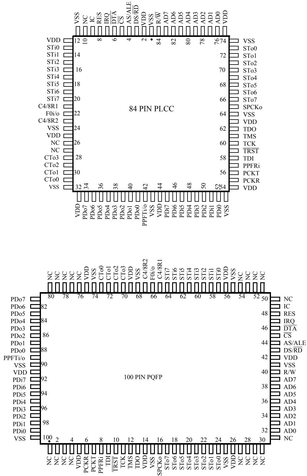
Figure 2 - Pin Connections
