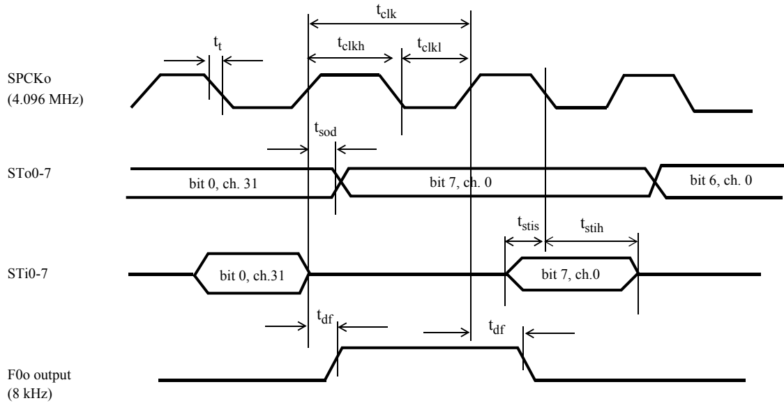
Serial Port with Positive Polarity F0 (GCI)
