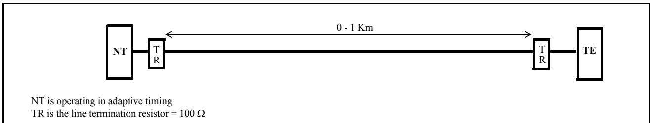
Figure 8 - Point-to-Point Configuration
