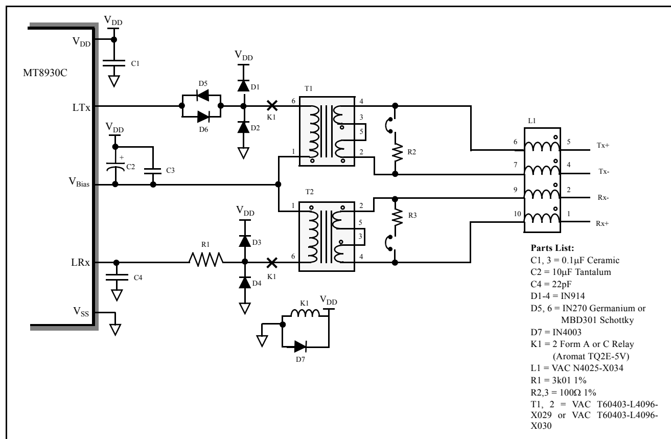
Figure 22 - ETS 300-012 NT &amp; TE Line Interface for VAC X029 or X030
