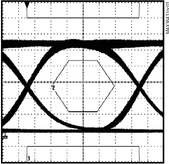
OPTICAL EYE DIAGRAM (1.25Gbps, 933MHz FILTER, PATTERN 2^{13}-1 + 80 CID)
