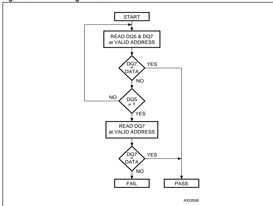
Figure 5. Data Polling flowchart
