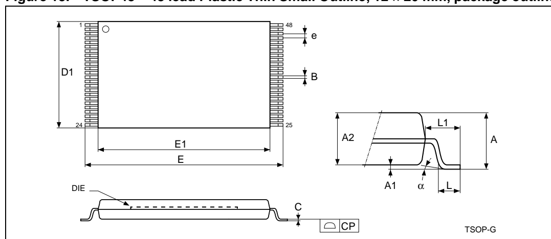
Figure 13. TSOP48 – 48 lead Plastic Thin Small Outline, 12 × 20 mm, package outline
