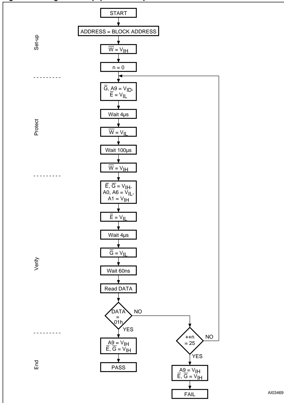
Figure 14. Programmer equipment block protect flowchart
