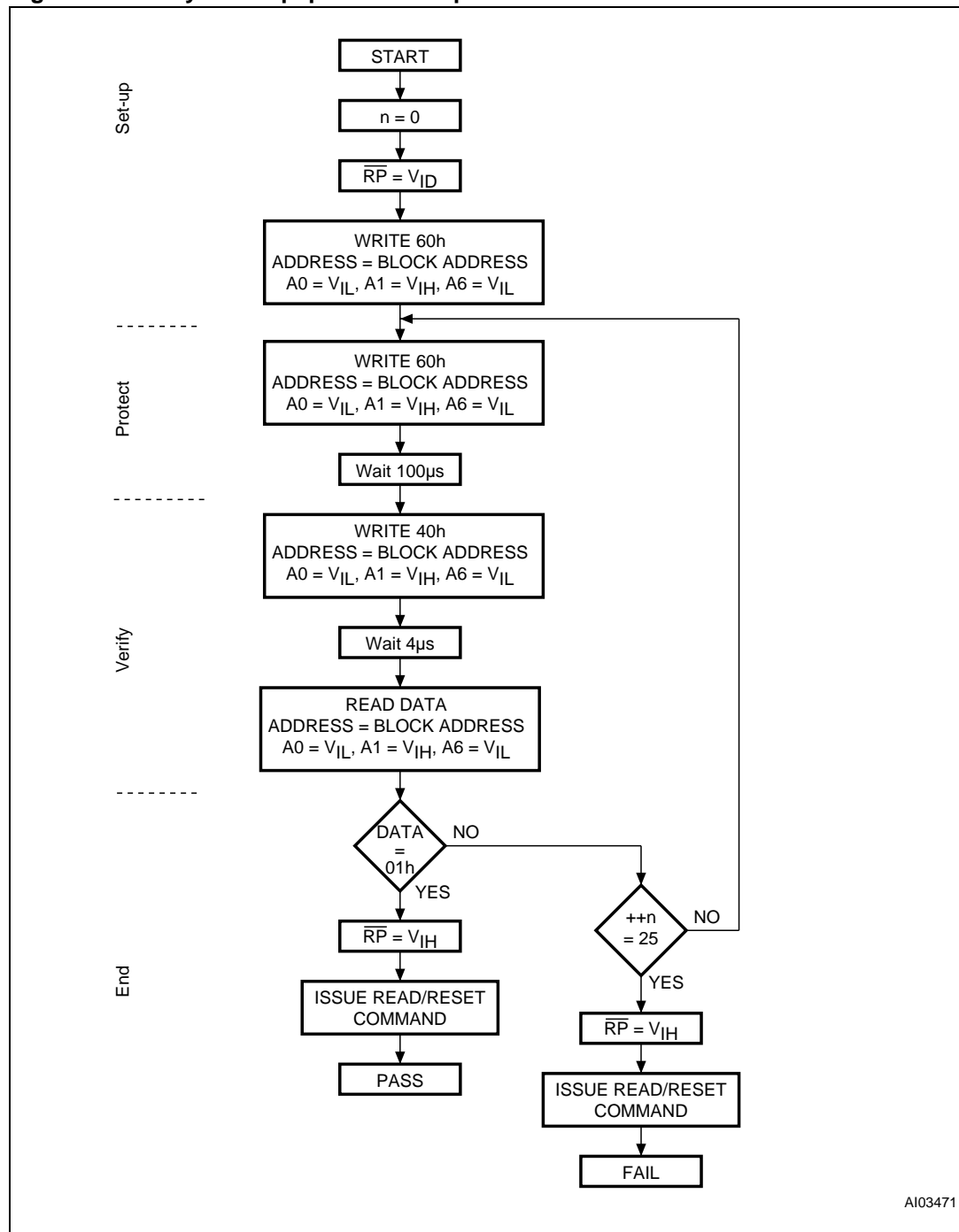
Figure 16. In-system equipment block protect flowchart
