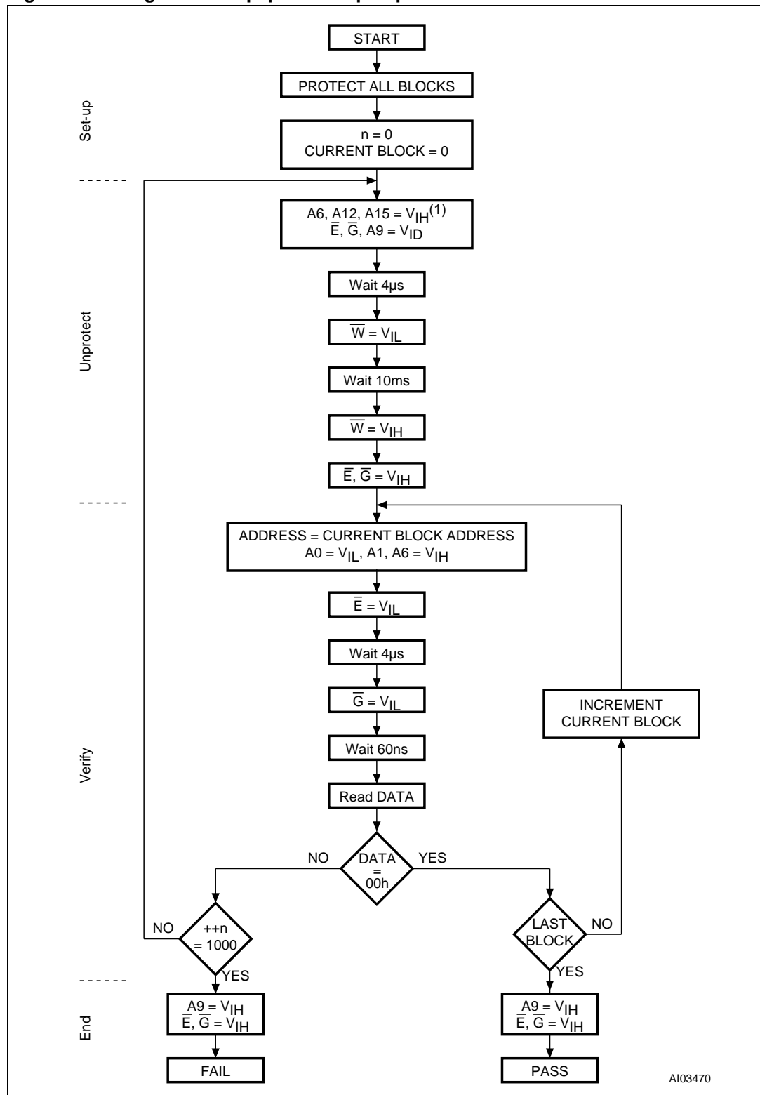
Figure 15. Programmer equipment chip unprotect flowchart
