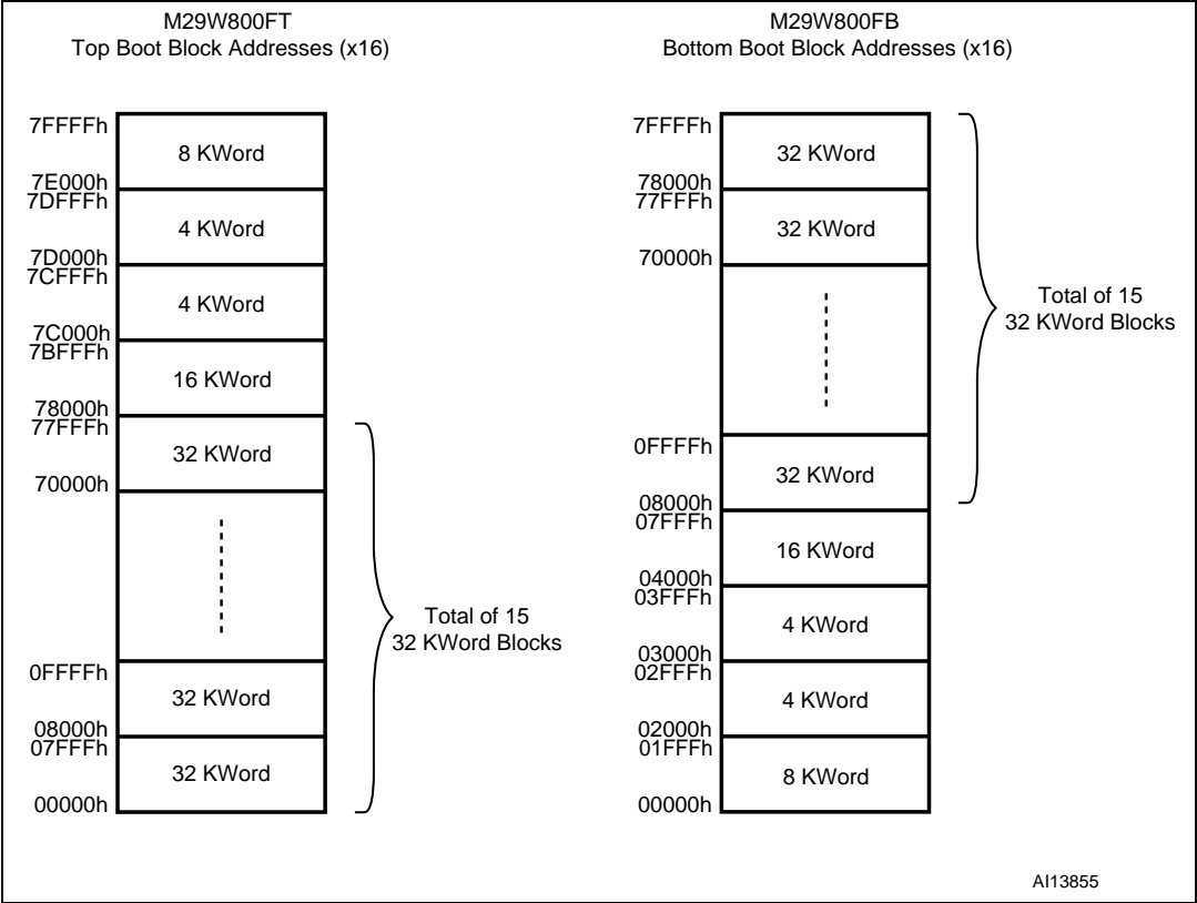
Figure 4. Block addresses (x16)
