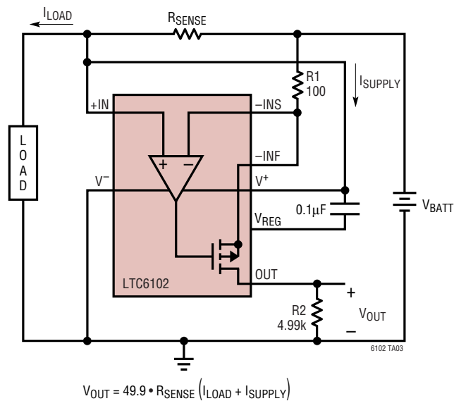
LTC6102 Monitors Its Own Supply Current
