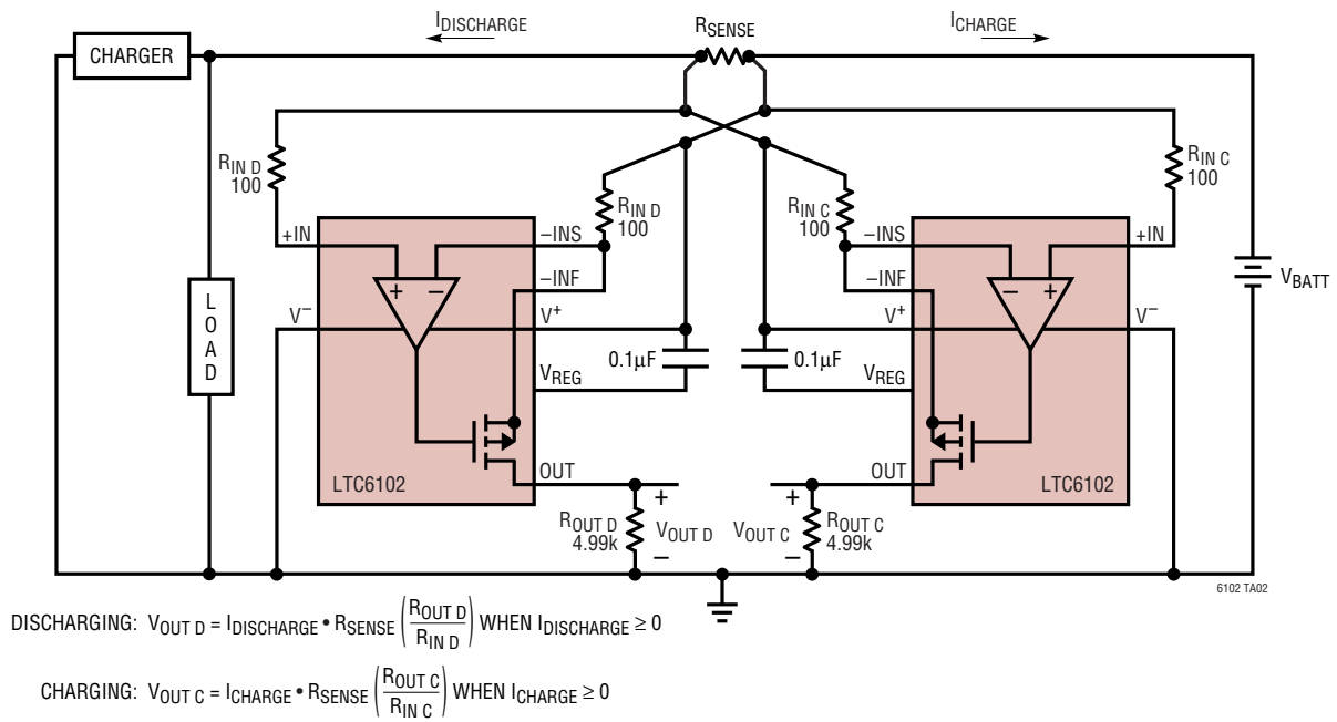
Bidirectional Current Sense Circuit with Separate Charge/Discharge Output
