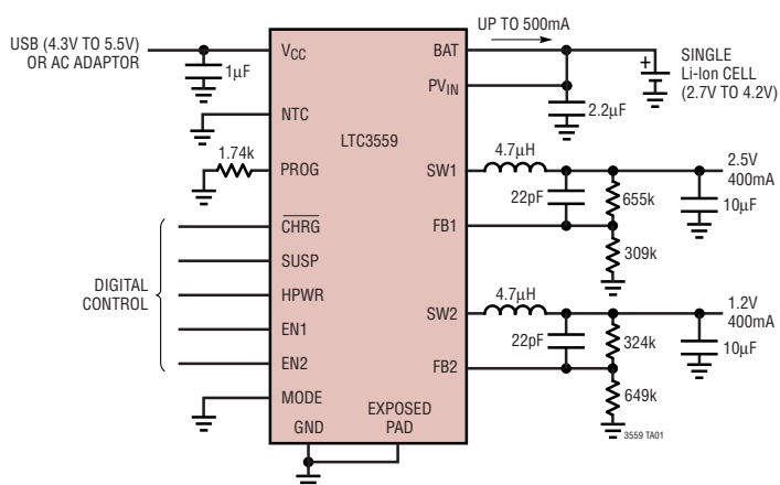
USB Charger Plus Dual Buck Regulators
