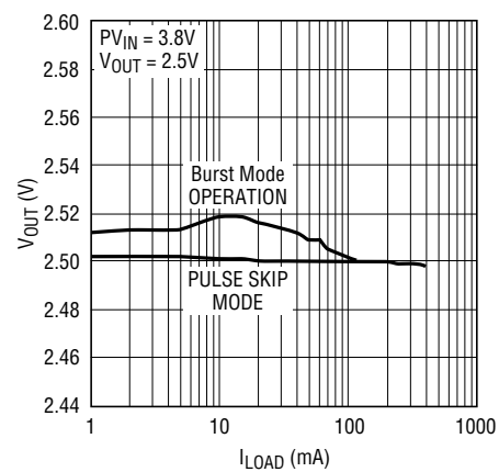
Buck Regulator Load Regulation
