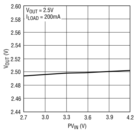
Buck Regulator Line Regulation
