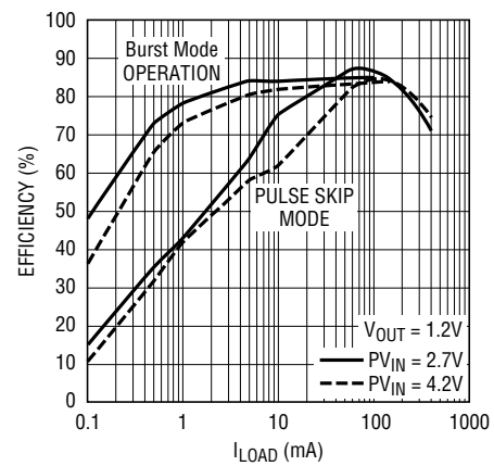
Buck Regulator Efficiency vs I_{LOAD}
