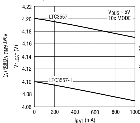
V_{FLOAT} Load Regulation
