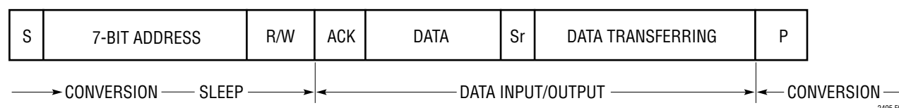
Figure 6. Conversion Sequence
