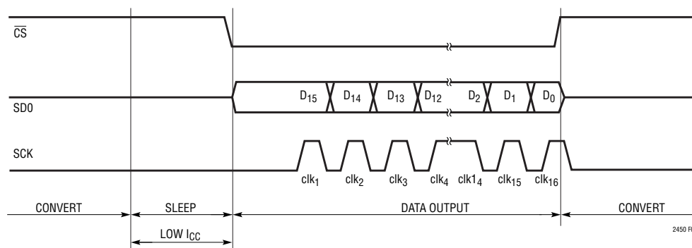
Figure 7. Idle-Low ( \overline{\text{CPOL}} = 0 ) Clock. \overline{\text{CS}} Triggers a New Conversion
