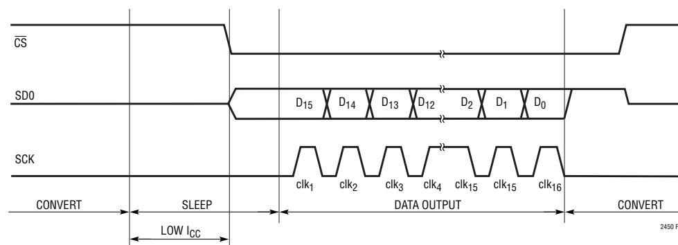
Figure 8. Idle-Low ( \overline{\text{CPOL}} = 0 ) Clock. The 16th SCK Falling Edge Triggers a New Conversion
