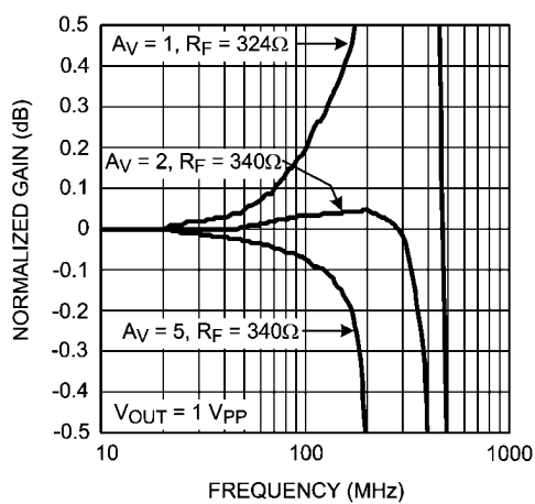
Gain Flatness
