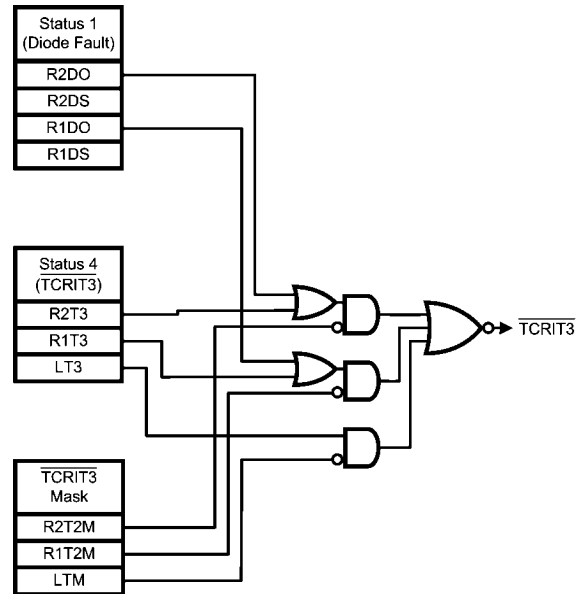
c) TCRIT3 Mask Register, Status Register 1 and 4, and TCRIT3 output logic diagram.
