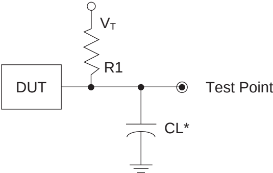
Figure 3-20. Output Test Load, LVTTTL and LVCMOS Standards
