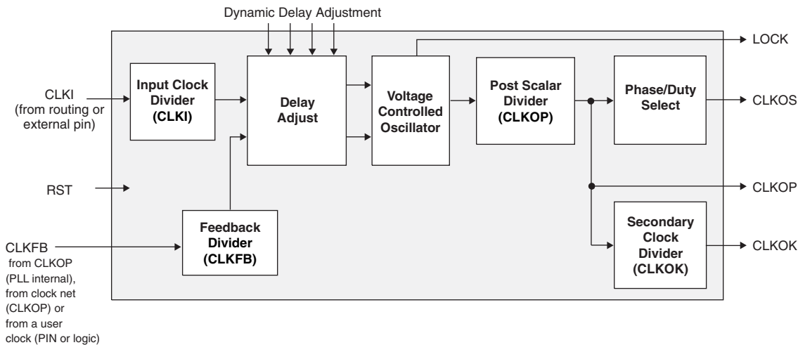
Figure 2-11. PLL Diagram
