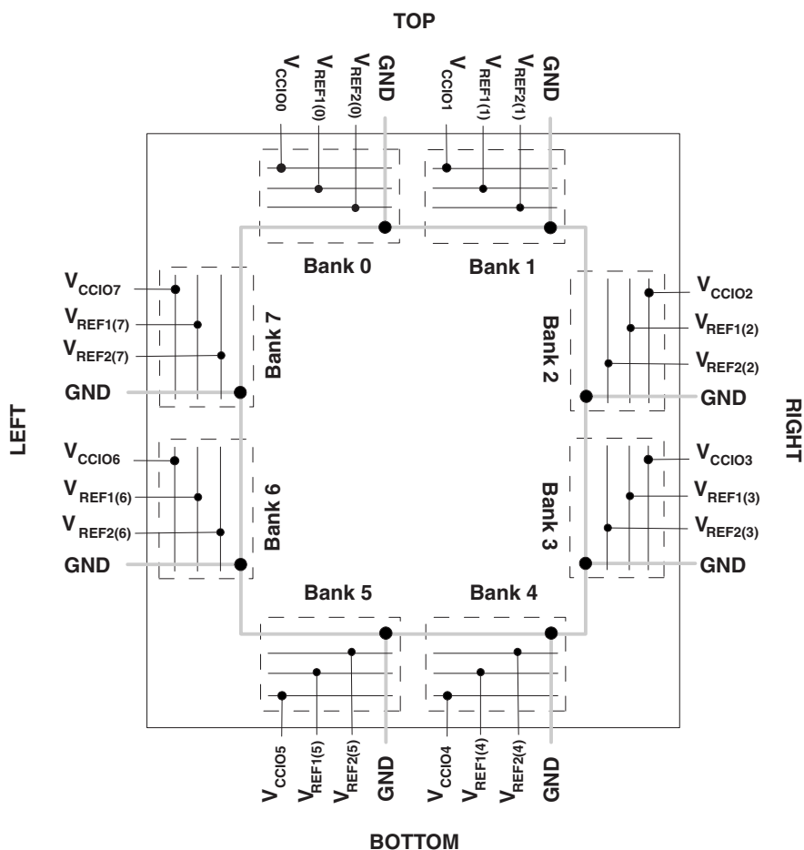
Figure 2-33. LatticeECP/EC Banks
