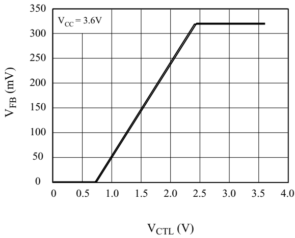
V_{FB} vs V_{CTL}
