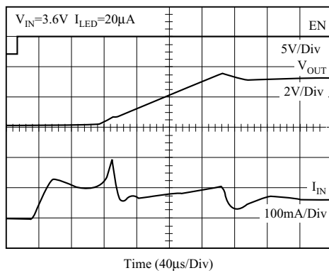
Inrush Current
