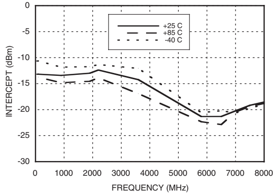
LOGOUT Intercept vs. Frequency, V_{CC} = 5V
