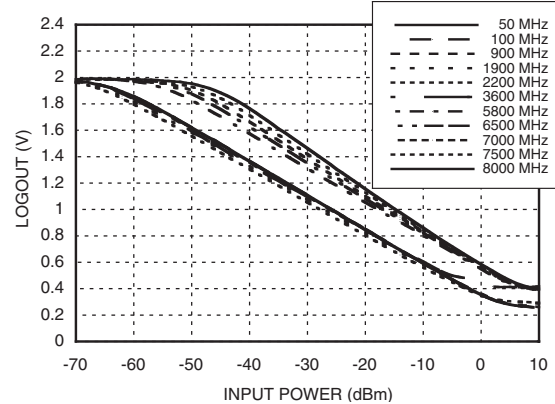
LOGOUT Voltage vs. Input Power & Frequency, T_A = +25C
