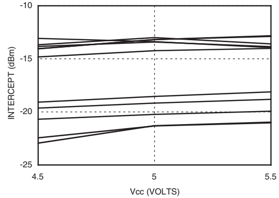
LOGOUT Intercept vs. Bias Voltage, T_A = +25C
