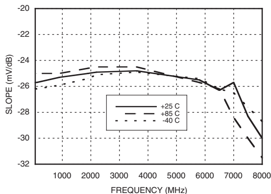
LOGOUT Slope vs. Frequency, V_{cc} = 5V
