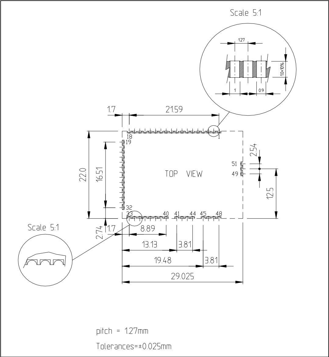
Figure 2. Mechanical dimensions
