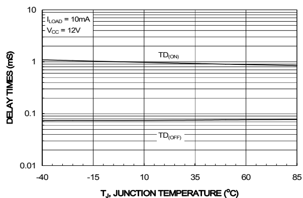
Figure 11. T_{ON}/T_{OFF} vs. Temperature
