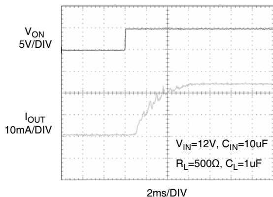
Figure 17. T_{ON} Response
