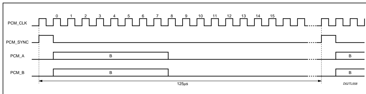
Figure 11. Linear mode
