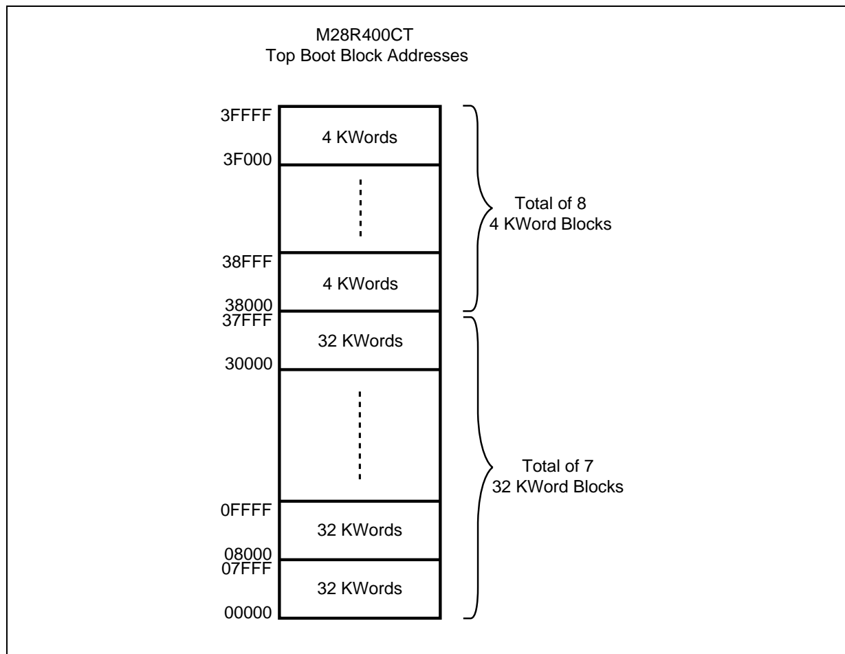
Figure 4. Block Addresses
