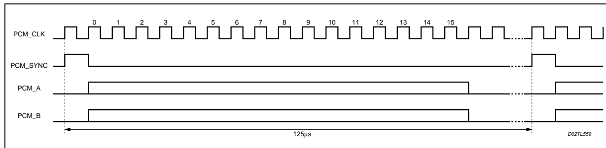
Figure 11. Linear mode
