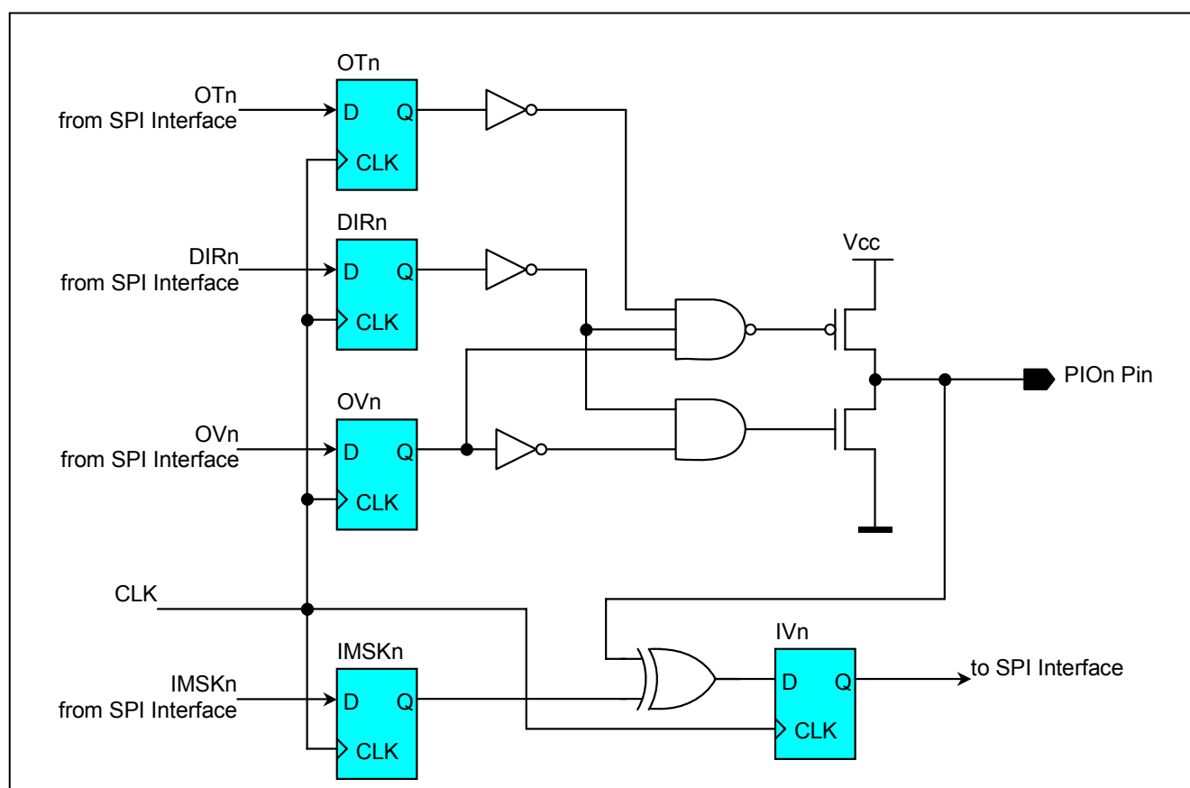
Figure 4. PIO Simplified Schematic
