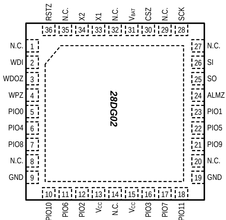
Thin 36-Lead 6mm x 6mm QFN (Top View) Package Outline Drawing 21-0141
