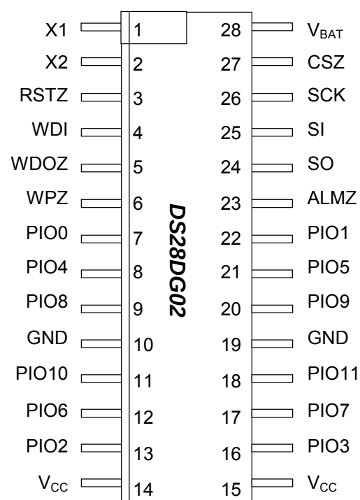
4.4mm 28-Lead TSSOP (Top View) Package Outline Drawing 21-0108
