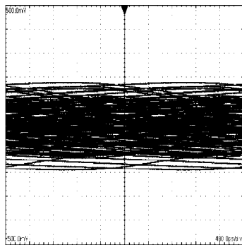
A 0.5 Gbps NRZ PRBS-7 After 100m CAT5e H:100 mV / DIV, V:400 ps / DIV
