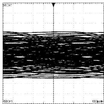
A 1.5 Gbps NRZ PRBS-7 After 200m Belden 9914 H:100 mV / DIV, V:100 ps / DIV
