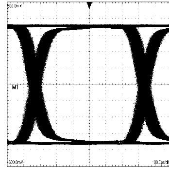
An Equalized 1.5 Gbps NRZ PRBS-7 After 25m CAT5e H:100 mV / DIV, V:100 ps / DIV
