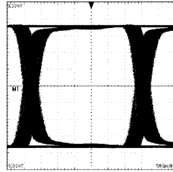
An Equalized 1.0 Gbps NRZ PRBS-7 After 50m CAT5e H:100 mV / DIV, V:150 ps / DIV
