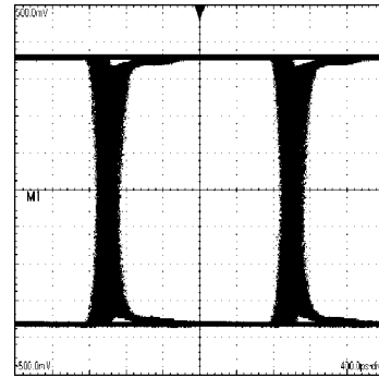
An Equalized 0.5 Gbps NRZ PRBS-7 After 100m CAT5e H:100 mV / DIV, V:400 ps / DIV
