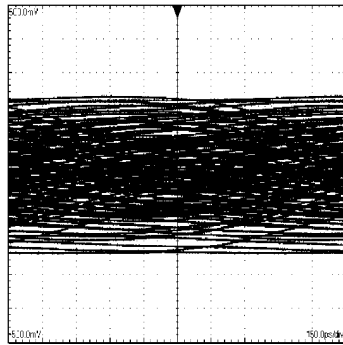
A 1.0 Gbps NRZ PRBS-7 After 50m CAT5e H:100 mV / DIV, V:150 ps / DIV
