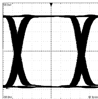
An Equalized 1.5 Gbps NRZ PRBS-7 After 200m Belden 9914, H:100 mV / DIV, V:100 ps / DIV
