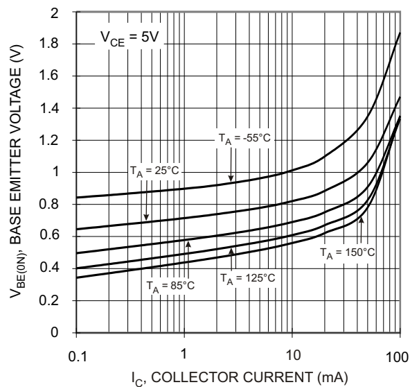
Fig. 9 V_{BE(ON)} vs. I_C
