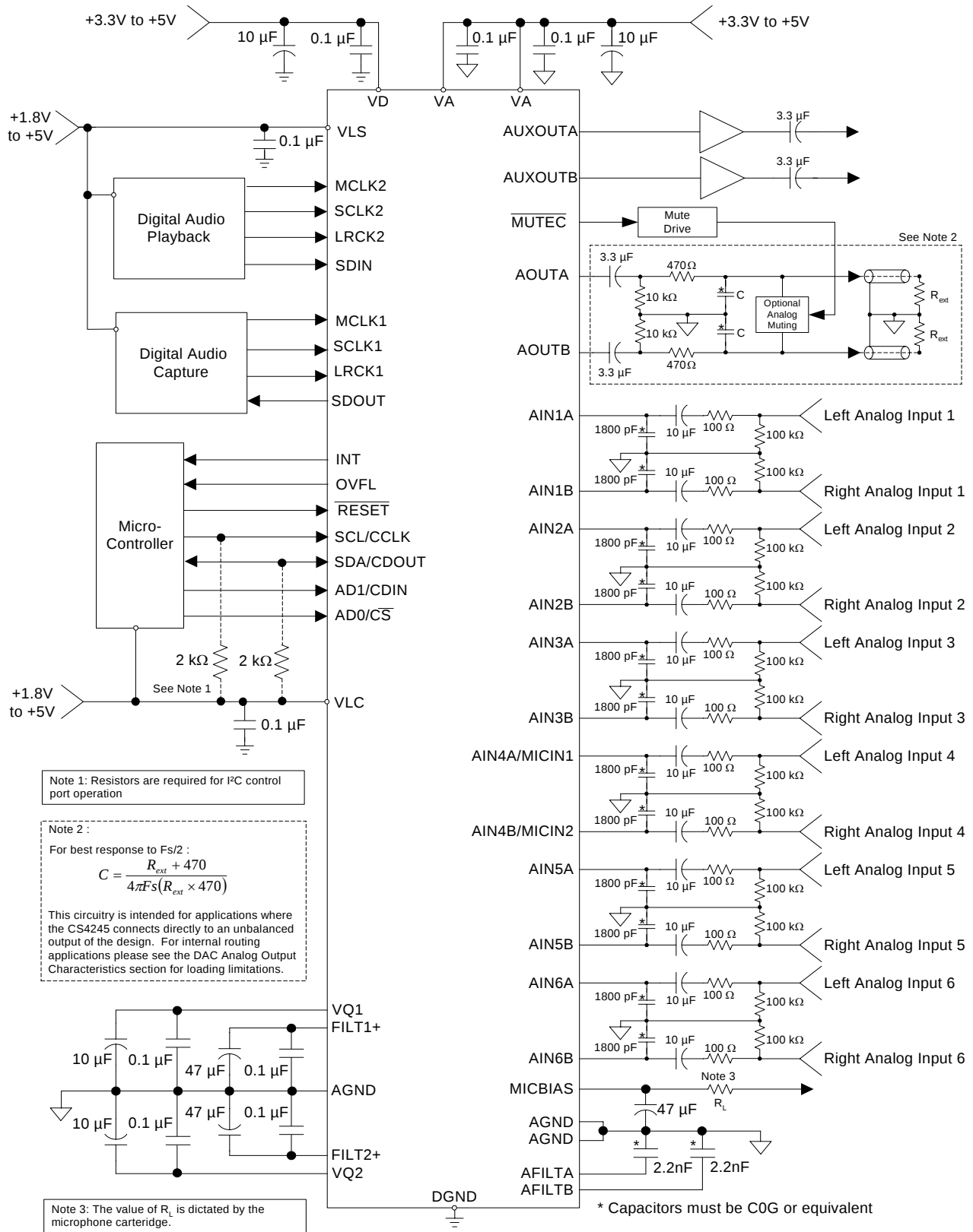
Figure 12. Typical Connection Diagram
