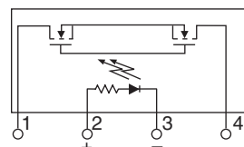
CPC1218Y Pinout
