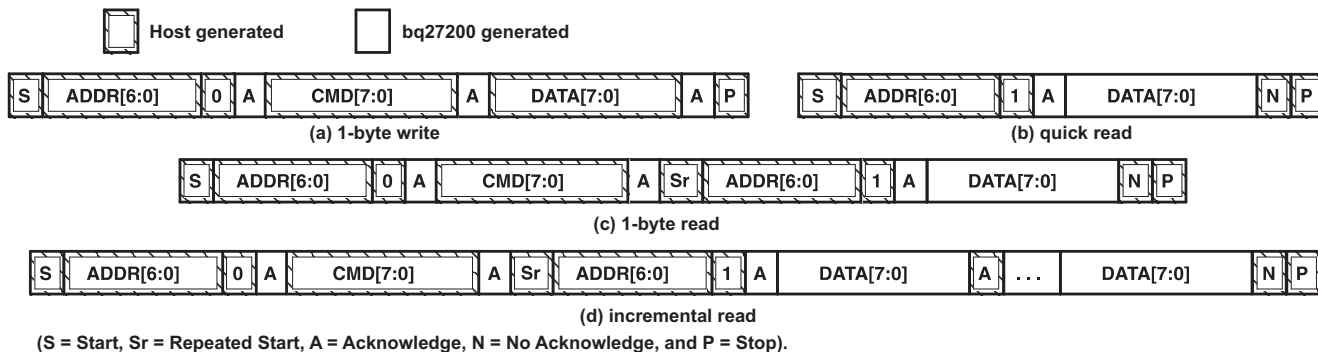
Figure 6-1. Supported I 2 C Formats
