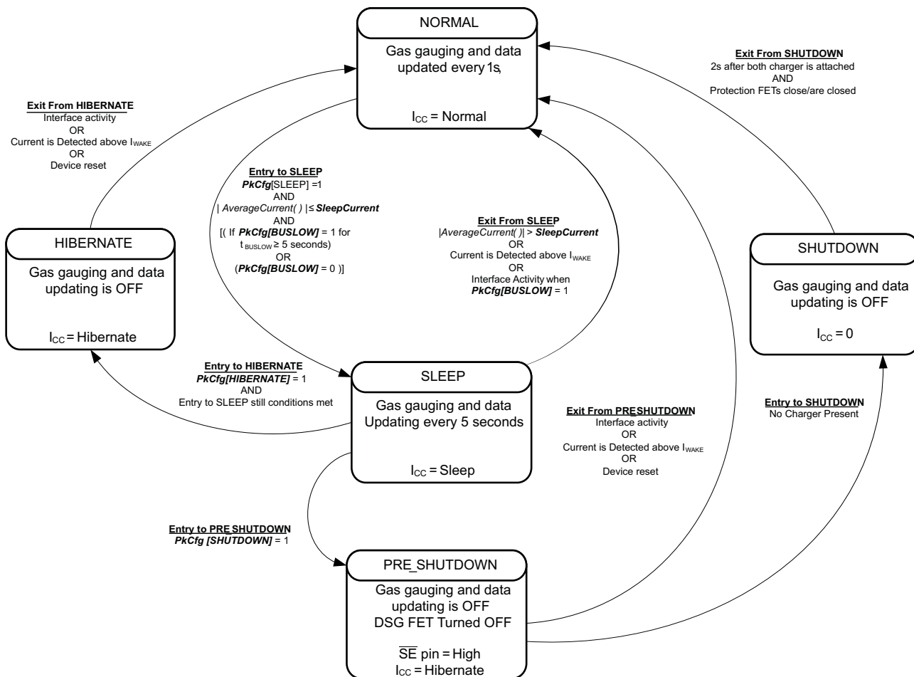
Figure 5-1. Power Mode Diagram
