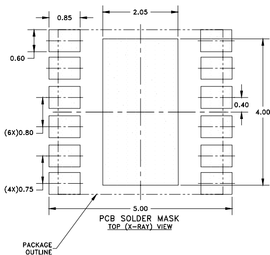
Figure 17: Land Pattern
