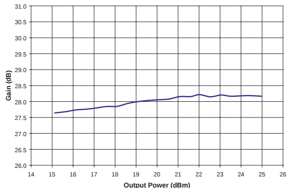
Figure 3: Gain vs. Output Power (T_C = +25^\circ\text{C}, V_{CC} = +6.0\text{ V}, V_{BIAS} = +3.0\text{ V}, f = 3.7\text{ GHz}, 54\text{ Mbps OFDM Modulation})
