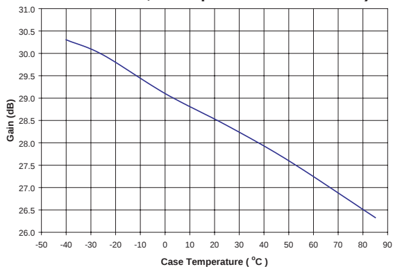
Figure 13: Gain vs. Case Temperature ( V_{CC} = +6.0\text{ V} , V_{BIAS} = +3.0\text{ V} , f = 3.7\text{ GHz} , P_{OUT} = +23\text{ dBm} , 54 Mbps OFDM Modulation)
