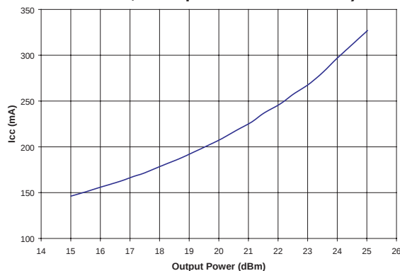
Figure 14: Supply Current vs. Output Power ( T_C = +25\text{ }^{\circ}\text{C} , V_{CC} = +6.0\text{ V} , V_{BIAS} = +3.0\text{ V} , f = 3.7\text{ GHz} , 54 Mbps OFDM Modulation)
