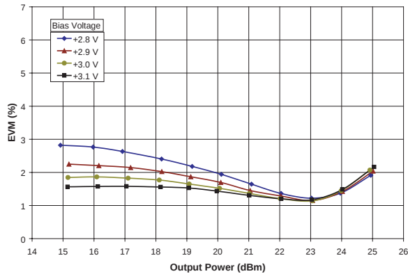
Figure 9: Effects of Bias Voltage ( V_{BIAS} ) on EVM ( T_C = +25\text{ }^\circ\text{C} , V_{CC} = +6.0\text{ V} , f = 3.7\text{ GHz} , 54 Mbps OFDM Modulation, system EVM Approx. 0.8 %)
