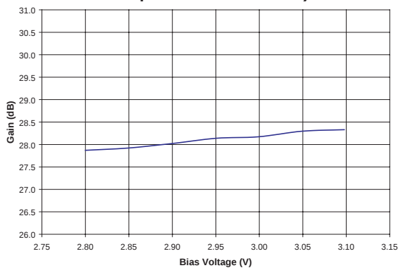
Figure 12: Gain vs. Bias Voltage ( V_{BIAS} ) ( T_C = +25\text{ }^{\circ}\text{C} , V_{CC} = +6.0\text{ V} , f = 3.7\text{ GHz} , 54 Mbps OFDM Modulation)
