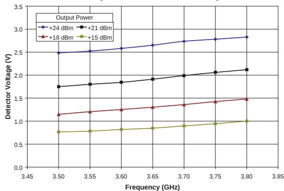
Figure 8: Detector Voltage vs. Frequency (T_C = +25^\circ\text{C}, V_{CC} = +6.0\text{ V}, V_{BIAS} = +3.0\text{ V}, 54\text{ Mbps OFDM Modulation})
