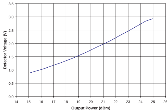
Figure 7: Detector Voltage vs. Output Power (T_C = +25^\circ\text{C}, V_{CC} = +6.0\text{ V}, V_{BIAS} = +3.0\text{ V}, f = 3.7\text{ GHz}, 54\text{ Mbps OFDM Modulation})
