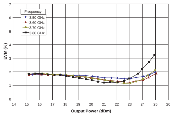
Figure 5: Uncorrected EVM vs. Output Power (T_C = +25^\circ\text{C}, V_{CC} = +6.0\text{ V}, V_{BIAS} = +3.0\text{ V}, 54\text{ Mbps} \text{OFDM Modulation, system EVM Approx. } 0.8\%)
