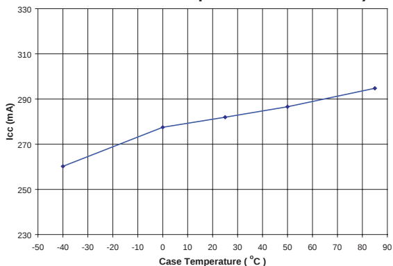
Figure 15: Supply Current vs. Case Temperature ( V_{CC} = +6.0\text{ V} , V_{BIAS} = +3.0\text{ V} , f = 3.7\text{ GHz} , P_{OUT} = +23\text{ dBm} , 54 Mbps OFDM Modulation)
