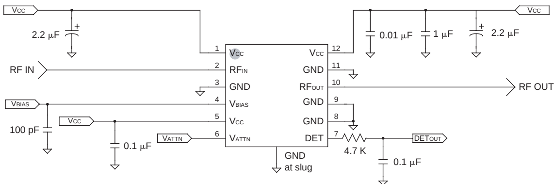
Figure 16: Application Circuit
